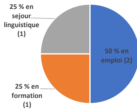
Insertion apprentissage
