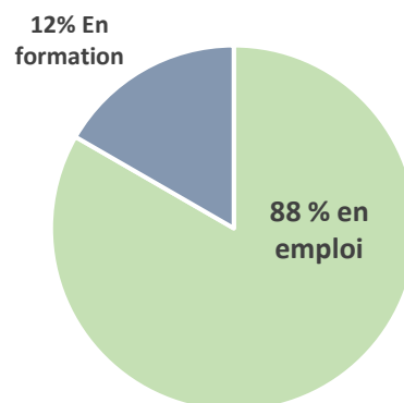
Insertion apprentissage
